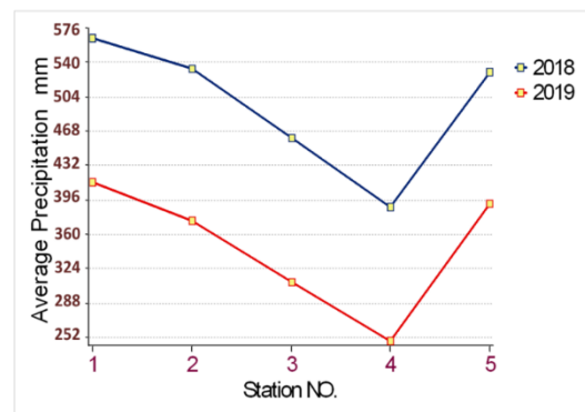
Fig. 2 Average annual precipitations during the study period.
