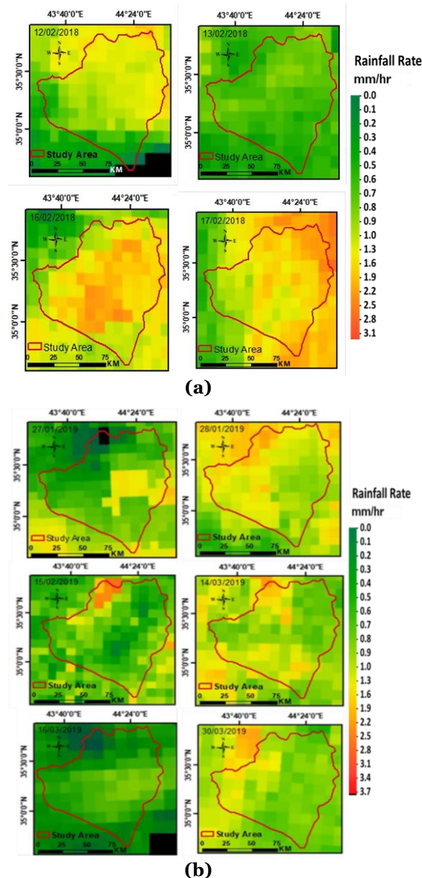
Fig. 6 Rainfall rate of full rainy days based on satellite images in (a) 2018 and (b) 2019.
