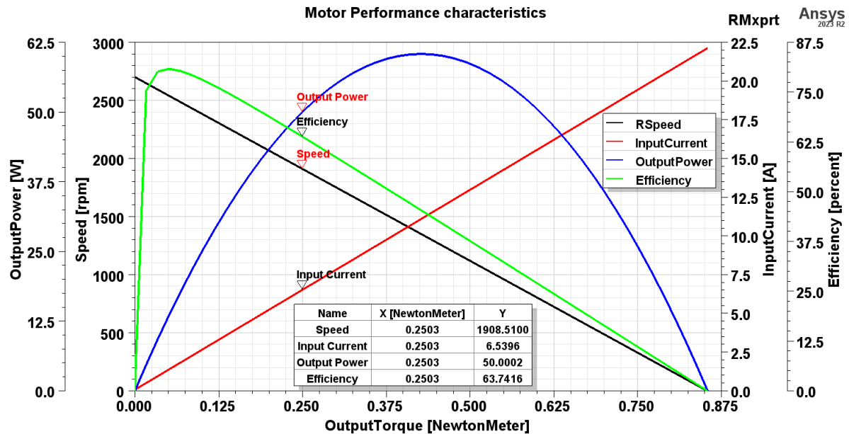
Fig. 15 Performance Curves of a PMDC Motor by RMxprrt.
