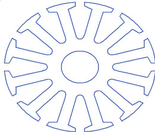
Fig. 6 Rotor Lamination Model by RMxpert.
