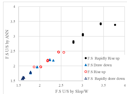
Fig 15. Model III Performance.
