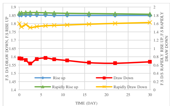
Fig 10. The change in the Downstream safety factor over time for model I.
