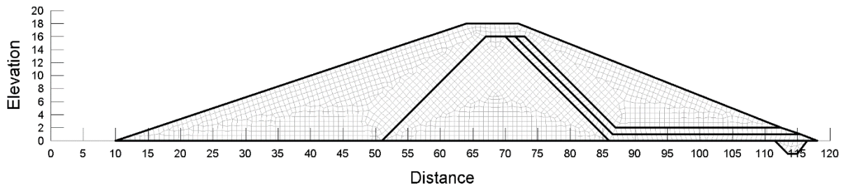
Fig. 2. The problem's finite element mesh
