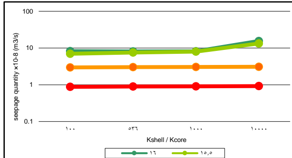
Fig. 4. The effect of changing ( k_{\text{shell}}/k_{\text{core}} ) on seepage quantity
