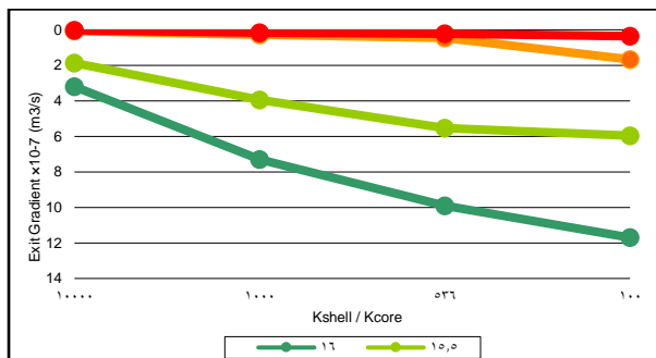
Fig. 5. The effect of changing ( k_{\text{shell}}/k_{\text{core}} ) on exit gradient
