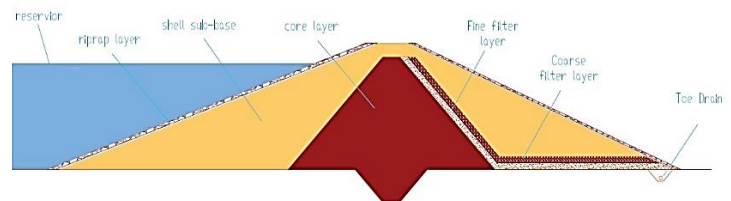
Fig. 1. The dam's body in cross-section
