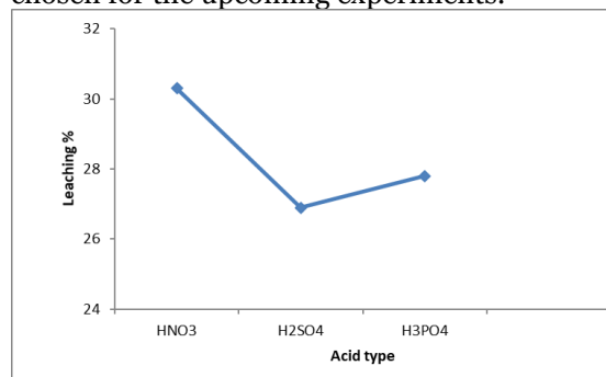
Fig.3. Effect of acid type on the leaching of titanium.
