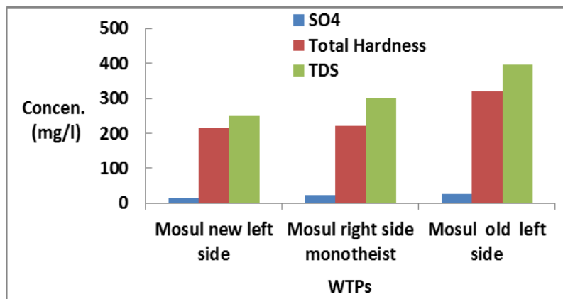
Fig. 7. Conc. of some effective parameters at the effluent of the three (WTPs)
