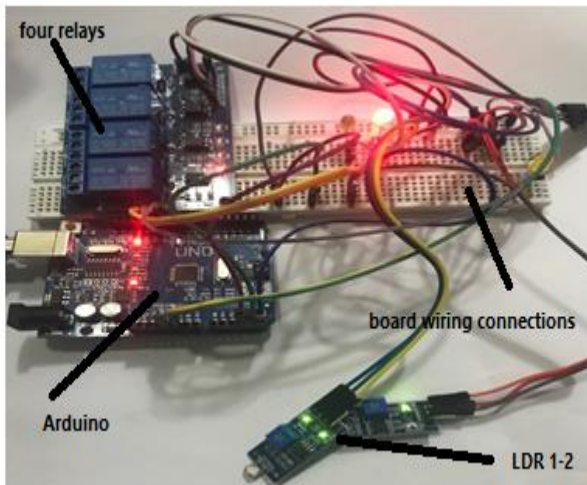
Fig.9. Control circuit
