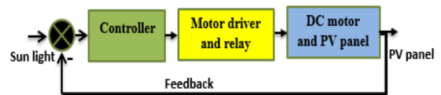
Fig.2. Block diagram of a Dual-Axis Tracking System [12]
