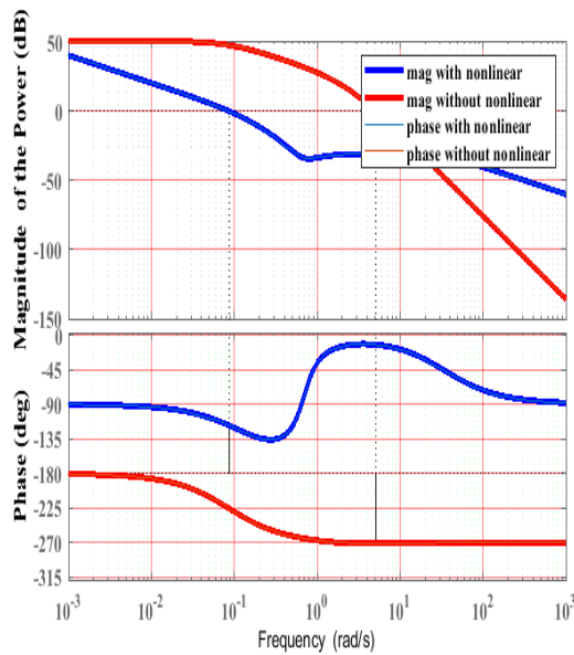
Fig.20. Bode plot of the complete system with and outshout the nonlinear element
