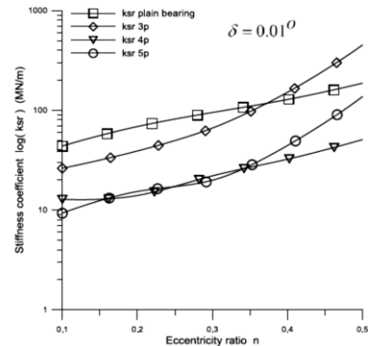
Fig. 9. Variation of K_{sr} for different number of pads against eccentricity ratio ( n ).
