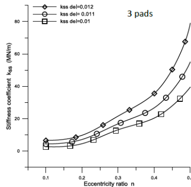
Fig. 13. Variation of K_{ss} for different pad angles against eccentricity ratio ( n ).
