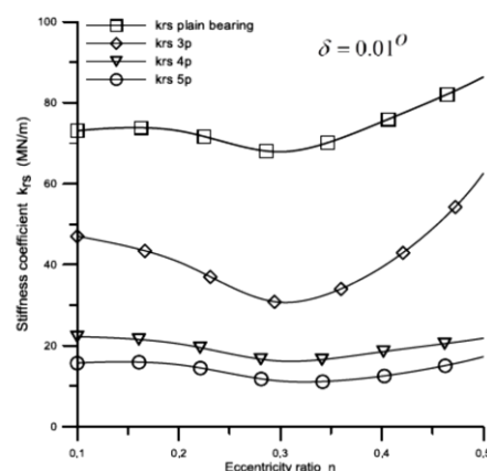
Fig. 11. Variation of K_{rs} for different number of pads against eccentricity ratio ( n ).
