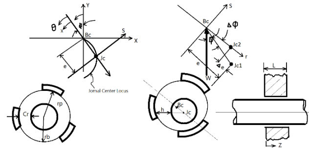
Fig. 1. Non-circular bearing.
