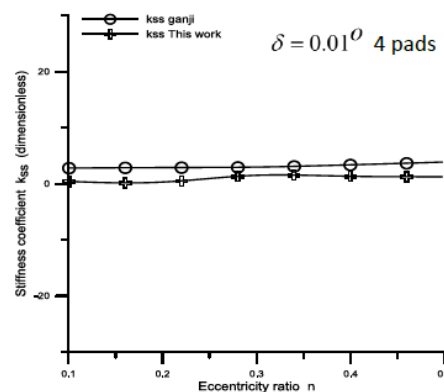
Fig. 4. Variation of K_{ss} with eccentricity ratio ( n ).
