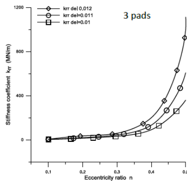
Fig. 12. Variation of K_{rr} for different pad angles against eccentricity ratio ( n ).
