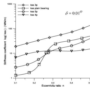
Fig. 10. Variation of K_{ss} for different number of pads against eccentricity ratio ( n ).
