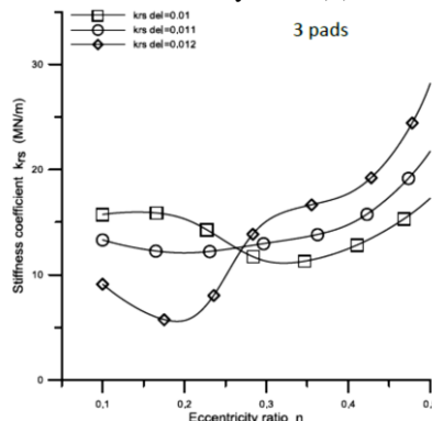
Fig. 15. Variation of K_{rs} for different pad angles against eccentricity ratio ( n ).
