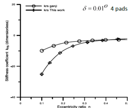
Fig. 5. Variation of K_{rs} with eccentricity ratio ( n ).
