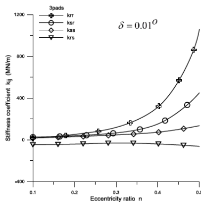
Fig. 7. Stiffness coefficients variation with the eccentricity ratio ( n ) for tilted pads bearing.
