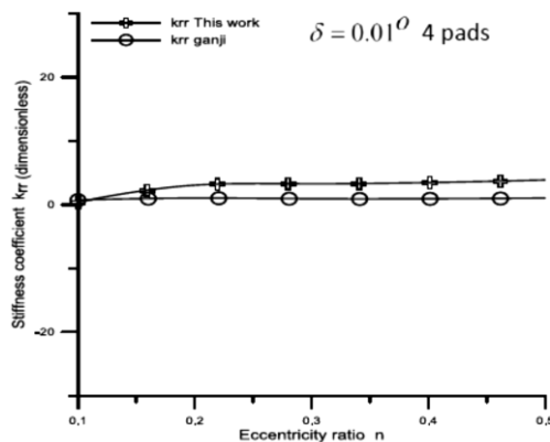
Fig. 2. Variation of K_{rr} with eccentricity ratio ( n ).
