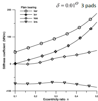
Fig. 6. Stiffness coefficients variation with the eccentricity ratio ( n ) for conventional bearing.
