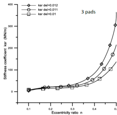
Fig. 14. Variation of K_{sr} for different pad angles against eccentricity ratio ( n ).
