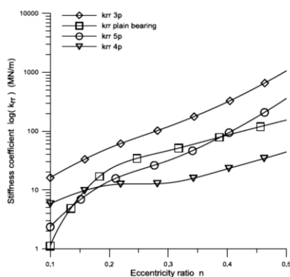
Fig. 8. Variation of K_{rr} for different number of pads against eccentricity ratio ( n ).
