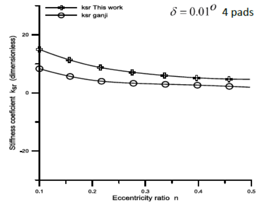
Fig. 3. Variation of K_{sr} with eccentricity ratio ( n ).
