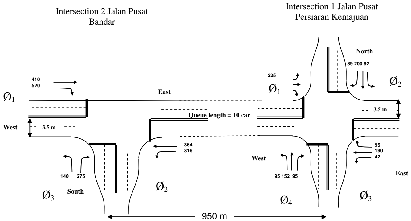
Fig.3 an illustration of two signalized intersections between Jalan Pusat Bandar And Persiaran Kemajuan
