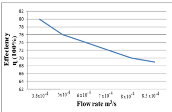
Fig. 3. Relationship between efficiency and flow rate of fluid.
