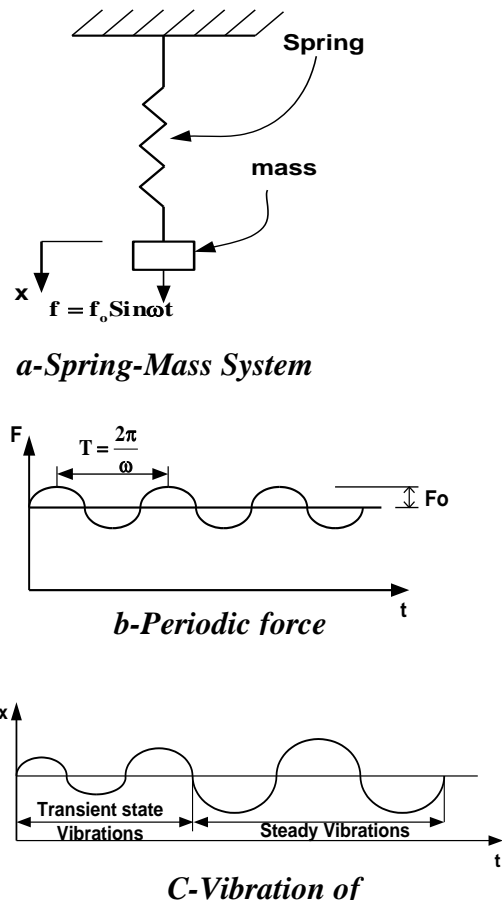
Fig.(1) Vibrations of a spring mass System
