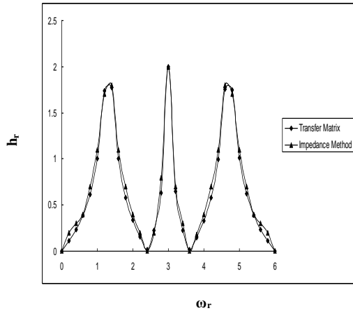
Fig.(12 a) Pressure Head Ratio Variation With Frequency Ratio
