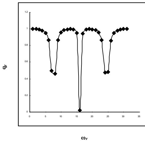
Fig.(12 b) Discharge Ratio Variation With Frequency Ratio
