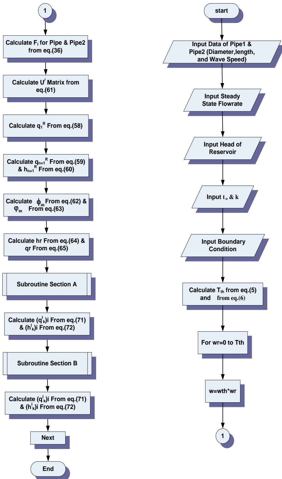
Fig.(11) Flow Chart of Computer Program Resonance
