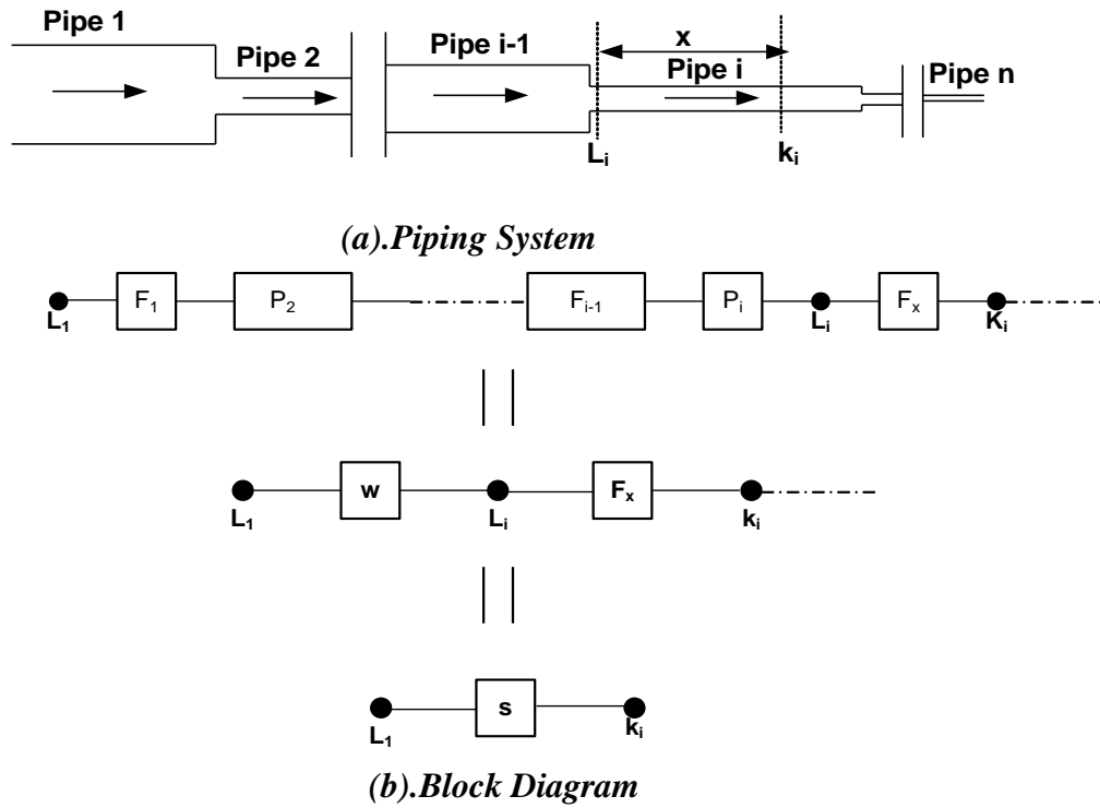
Fig.(9) Designation of k^{th} Section on i^{th} Pipe
