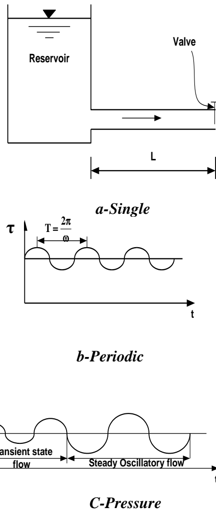
Fig.(2) Development of Steady-Oscillatory Flow in a Single Pipeline
