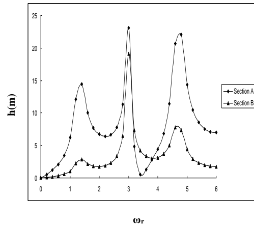
Fig.(13) Pressure Head Variation With Frequency Ratio at Section A&B
