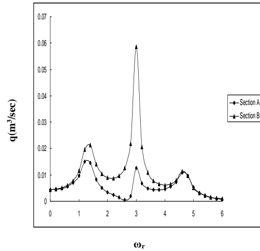
Fig.(14) Discharge Variation With Frequency Ratio at Section A&B
