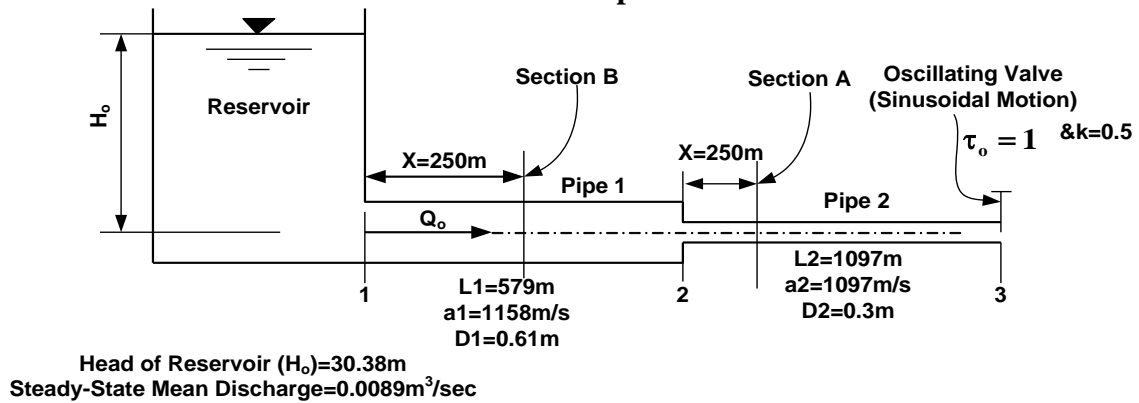
Figure(10a) Piping system
